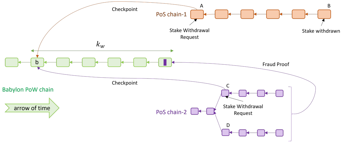
Figure 5: Delayed granting of withdrawal request and slashing. A validator for the PoS chain-1 sends a stake withdrawal request to its chain which is captured by the PoS block A. Block A is in turn checkpointed by the Babylon block b. This stake withdrawal request will only be granted and executed at a later PoS block B, where B is generated by a validator that observes the checkpoint of block A in block b become at least k_w deep in Babylon and that there is no fraud proof. On the other hand, the validator for the PoS chain-2 is not granted its withdrawal request and is slashed, since a fraud proof appears on Babylon before block b becomes k_w -deep.
